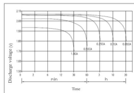
Discharge characteristics
